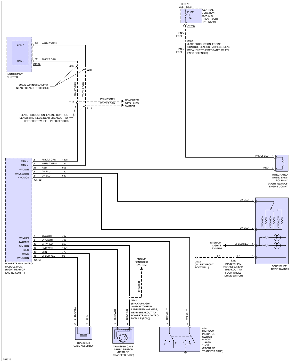
Fig 2: 4WD Circuit, Electronic
