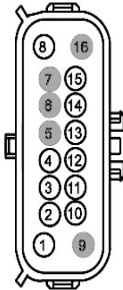
MALE Harness 12A581
